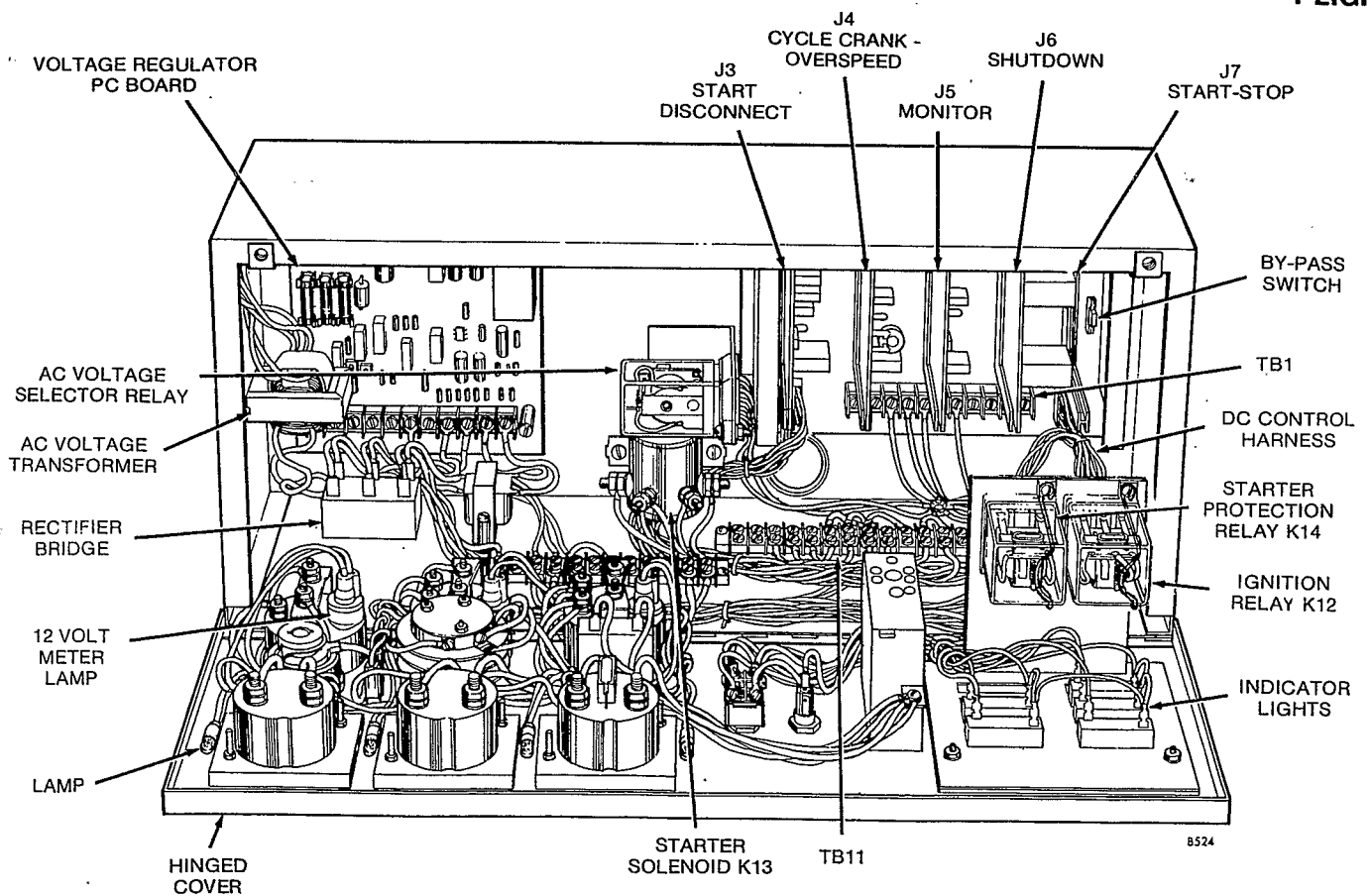
FIGURE 2. CONTROL PANEL INTERIORS
