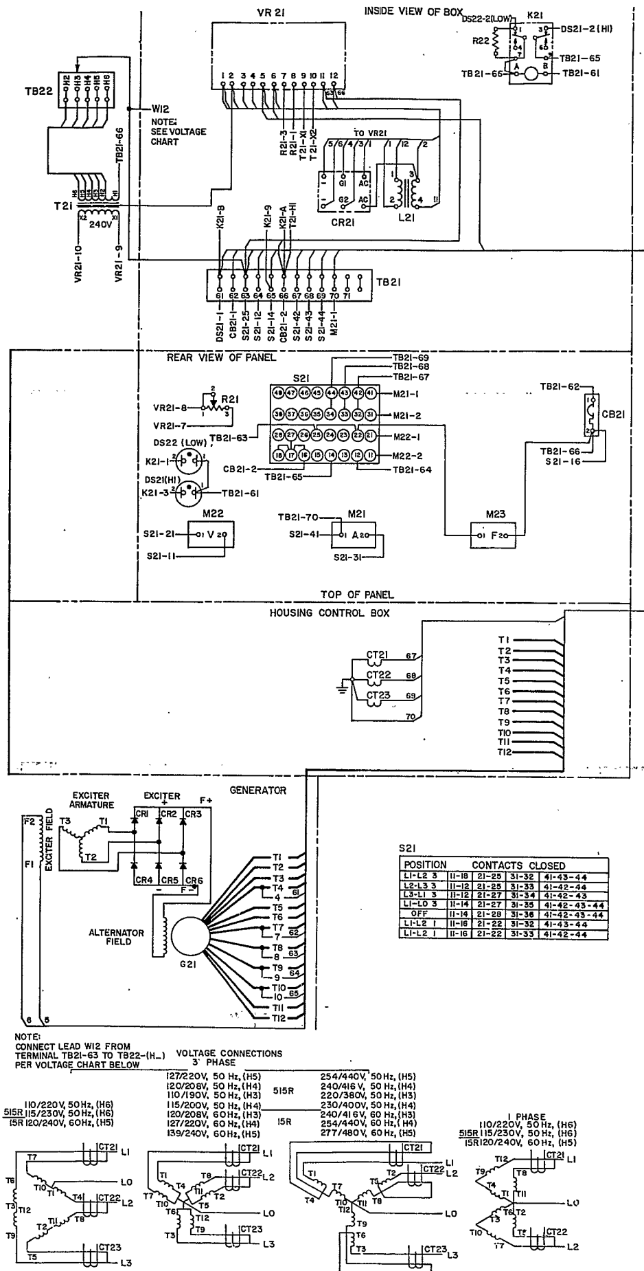
FIGURE 19. SK FIVE-LIGHT 3-PHASE, 60 Hz AC CONTROL 12-WIRE RECONNECTABLE (612-5433 SHEET 1)
