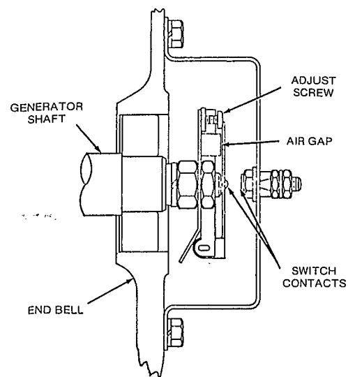
FIGURE 9. OVERSPEED SENSOR, OVERSPEED SWITCH
