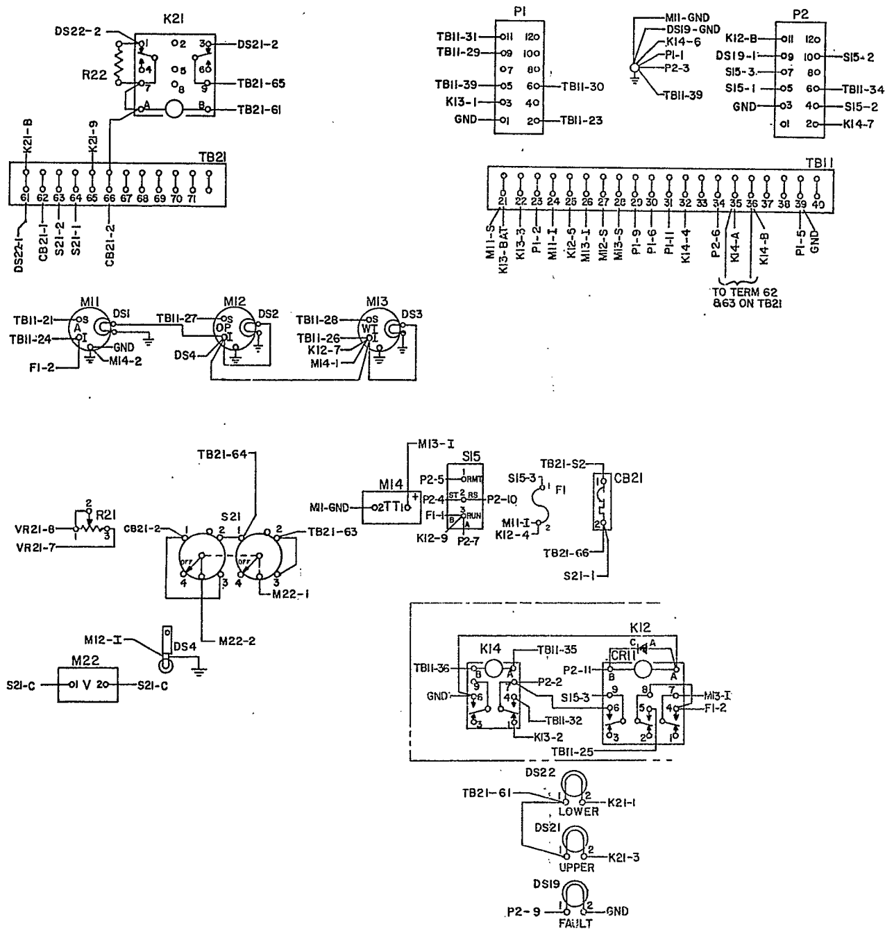
FIGURE 14. ONE-LIGHT CONTROL PANEL ASSEMBLY WIRING DIAGRAMS (300-1605)
