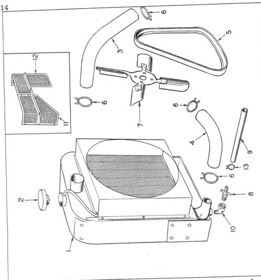
FIG. 18 - RADIATOR GROUP
