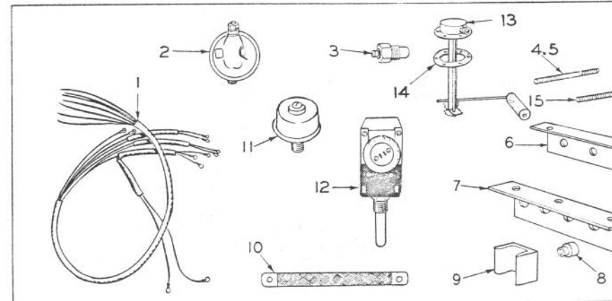
FIG. 19 - CONTROL ACCESSORIES GROUP
