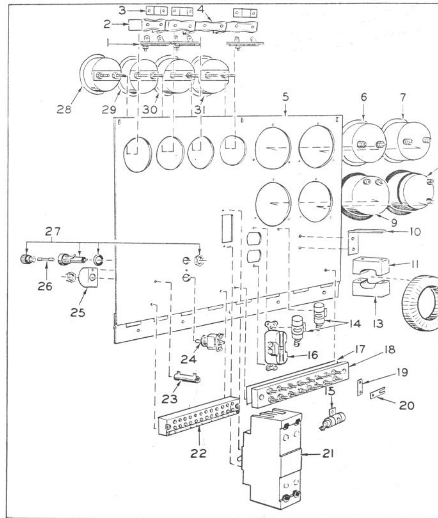
FIG. 20 - ELECTRICAL GROUP
