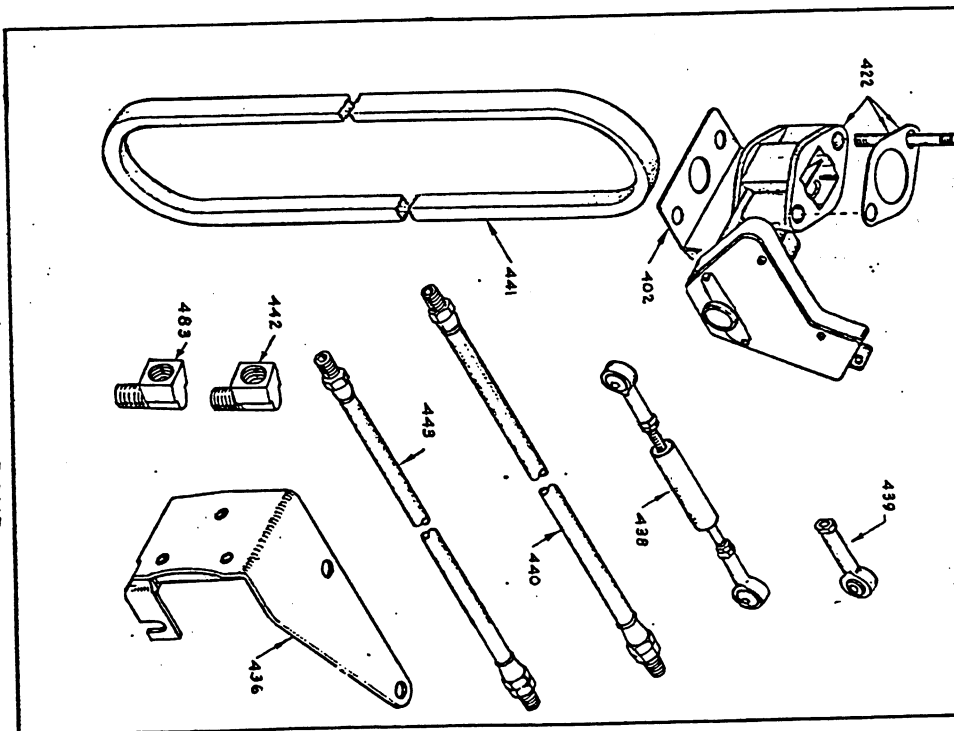
GOVERNOR MISC. GROUP FIG. 19
