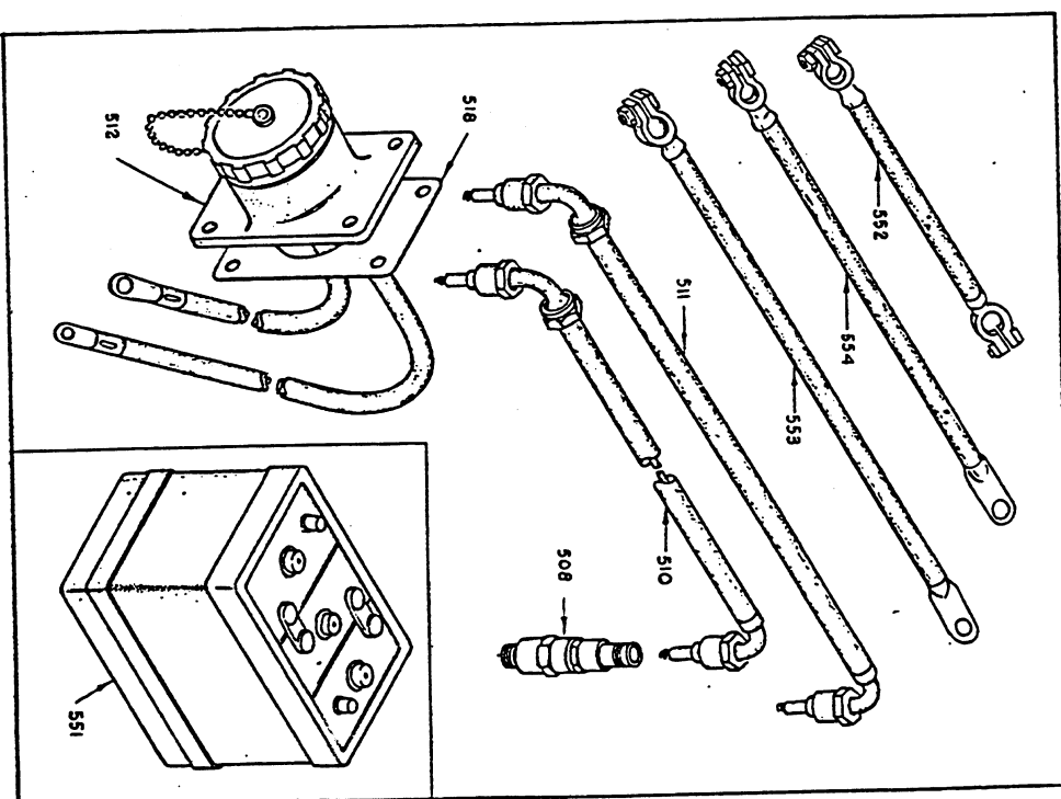
IGNITION GROUP FIG. 21
