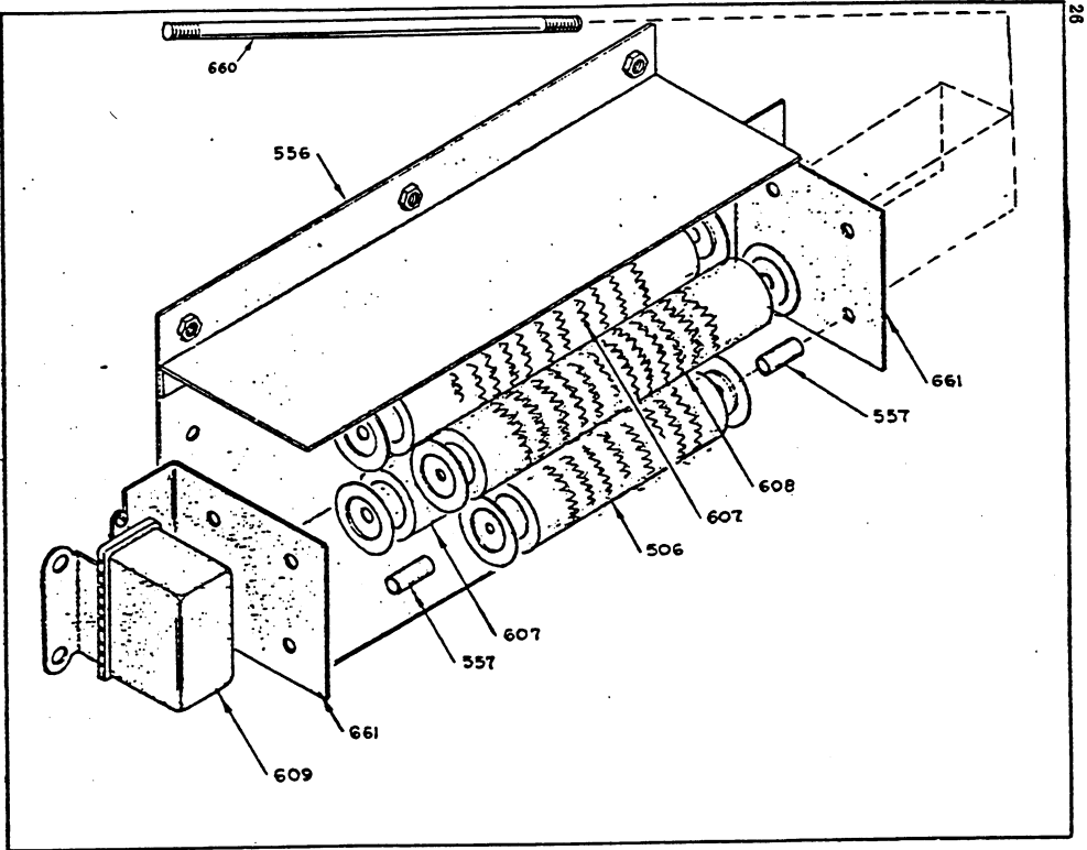
RESISTOR & VOLTAGE REGULATOR GROUP FIG. 26
