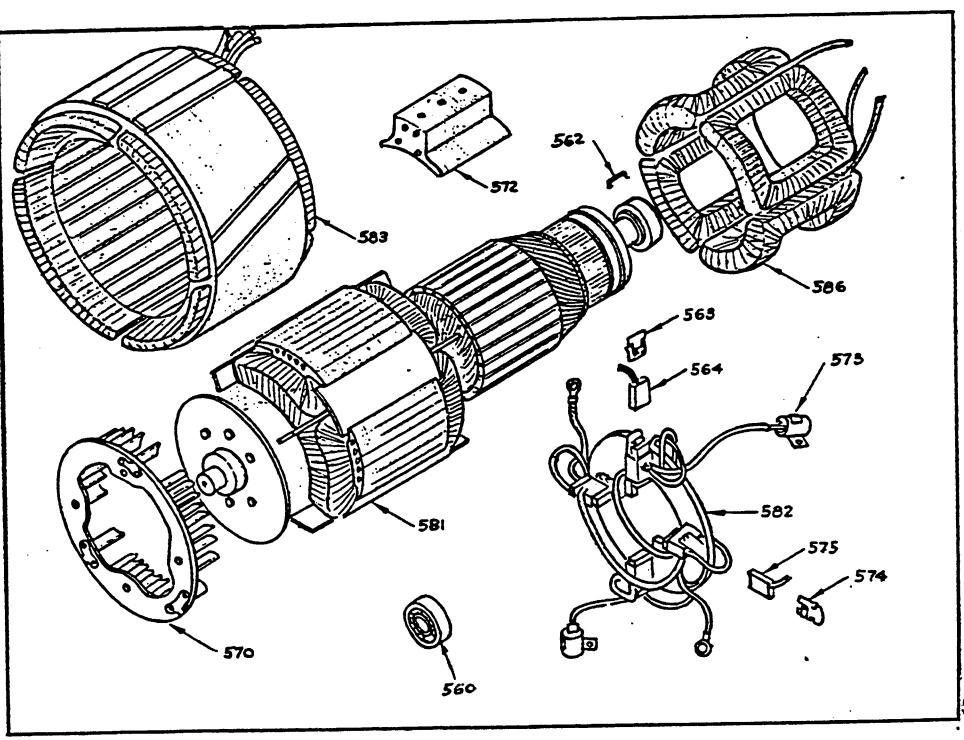
GENERATOR (INTERNAL) GROUP FIG. 23
