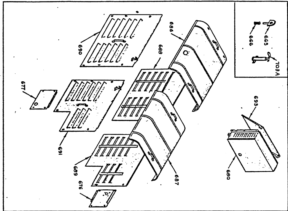
HOUSING PANEL GROUP FIG. 28
