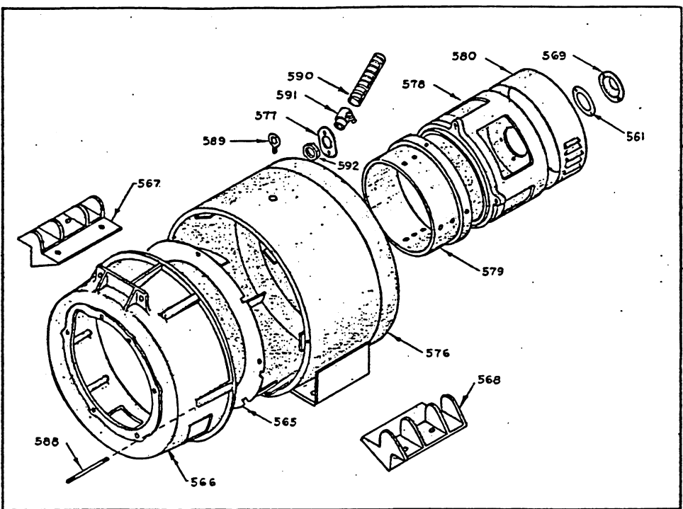
GENERATOR HOUSING GROUP FIG. 22
