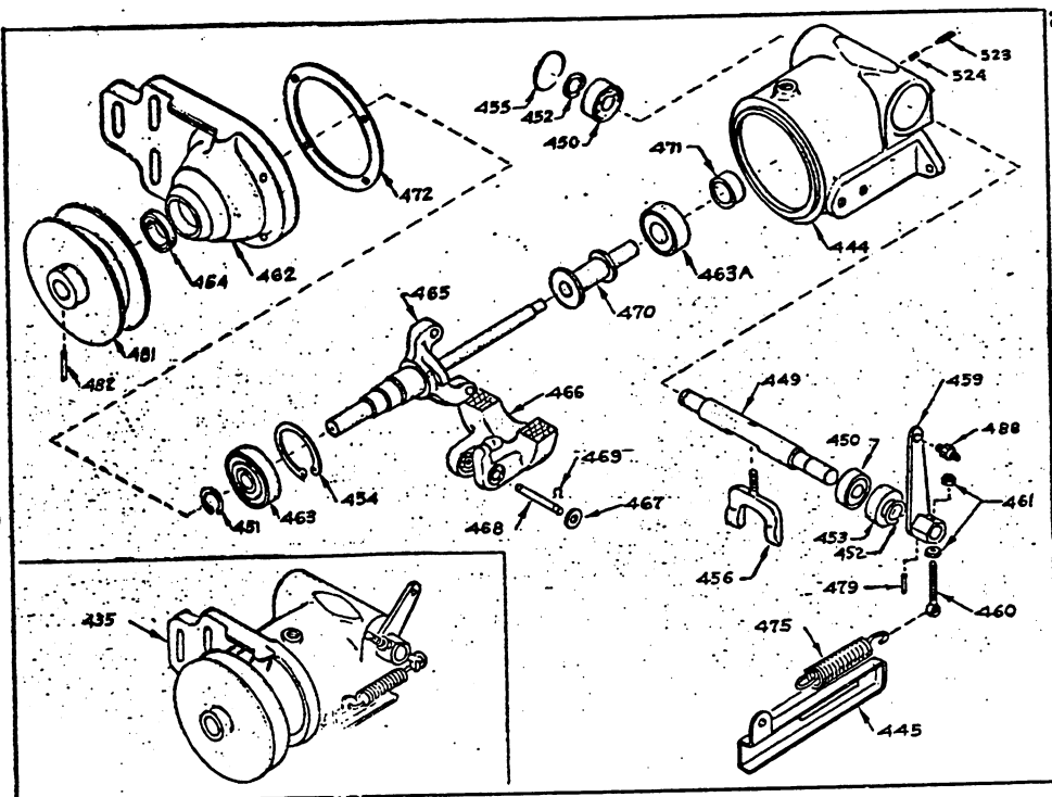
GOVERNOR GROUP FIG. 18
