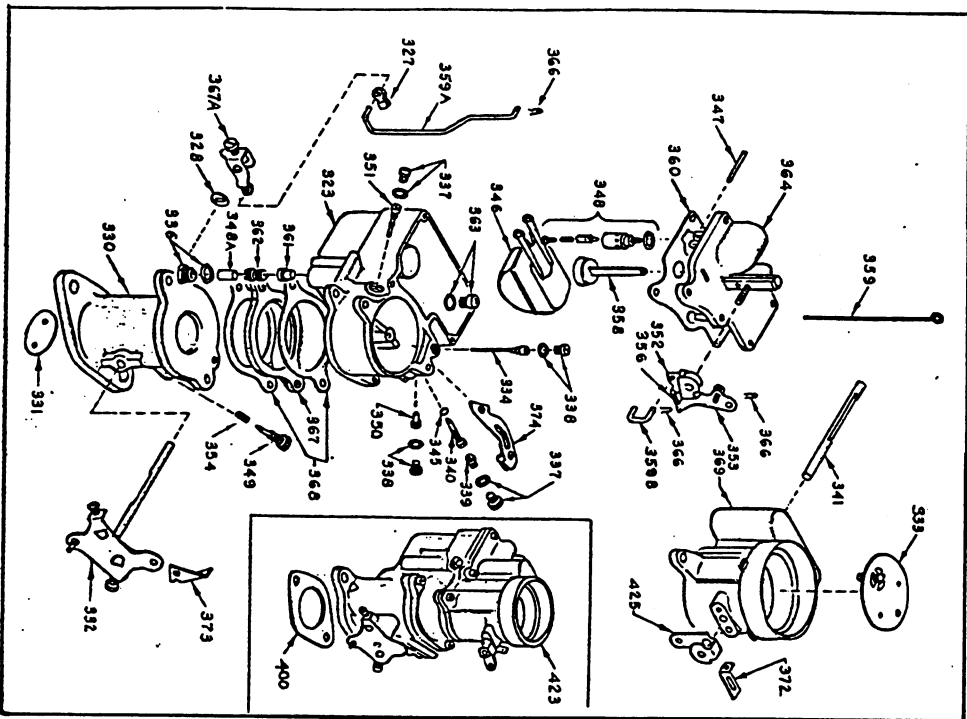
CARBURETOR GROUP FIG.14
