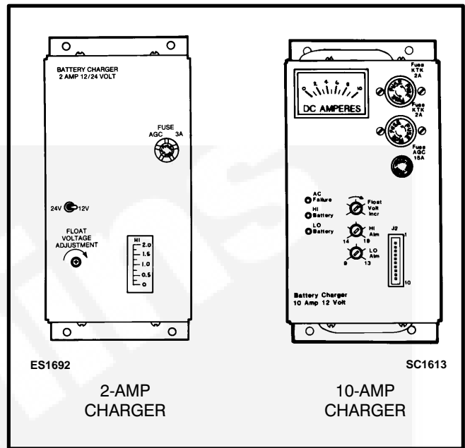
FIGURE 2-5. BATTERY CHARGER
