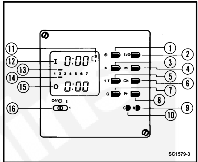
FIGURE 2-7. CHANGE-OVER CLOCK
