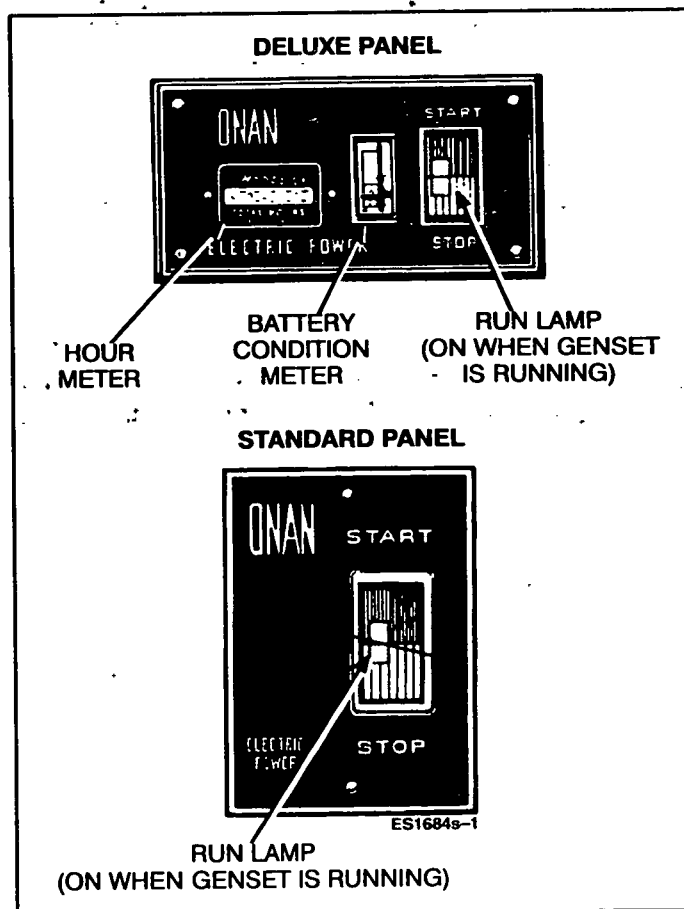
FIGURE 4. REMOTE CONTROL PANELS
