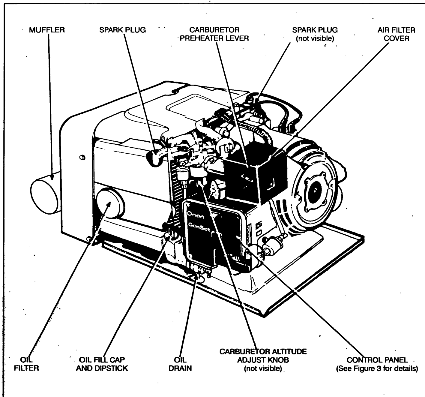
FIGURE 2. COMPONENT LOCATIONS
