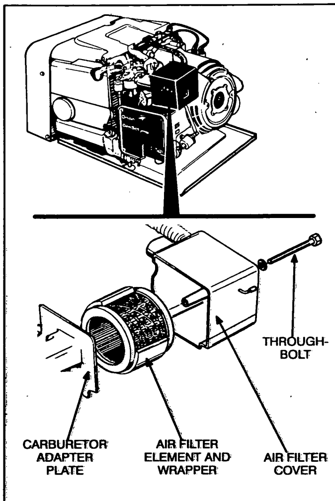
FIGURE 11. AIR FILTER ELEMENT AND WRAPPER
