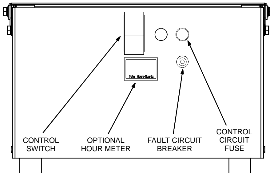
FIGURE 4-1. CONTROL PANEL
