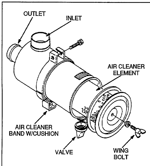
FIGURE 9. AIR CLEANER ASSEMBLY
