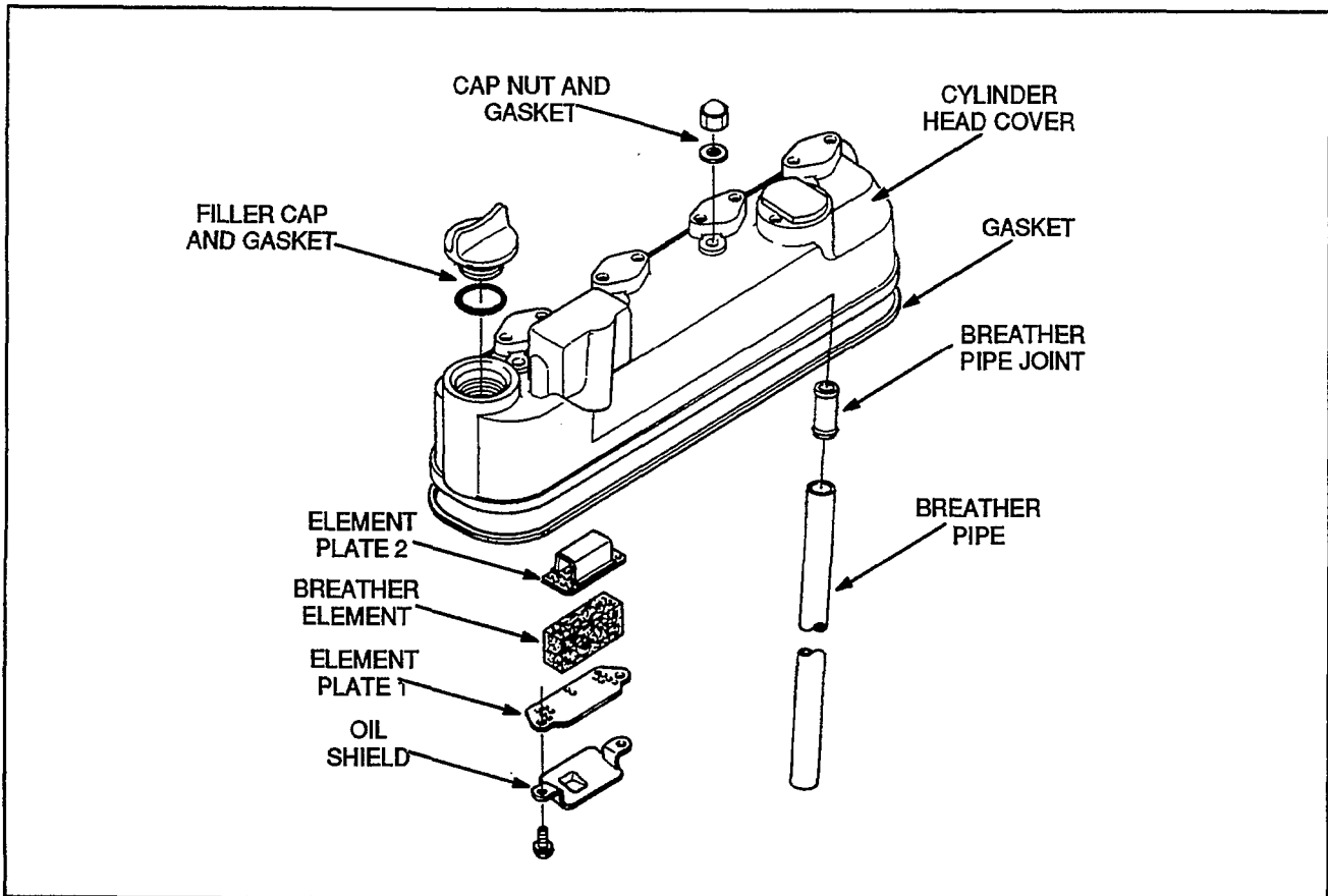
FIGURE 11. CRANKCASE BREATHER
