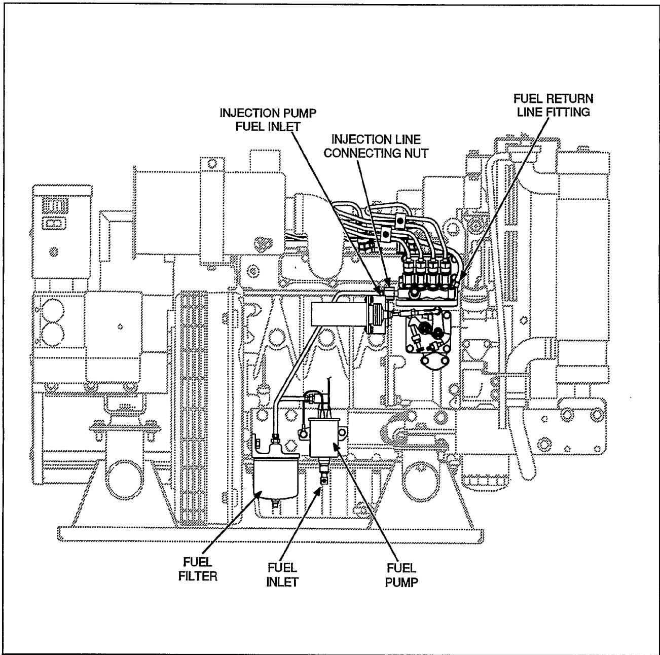
FIGURE 8. FUEL SYSTEM
