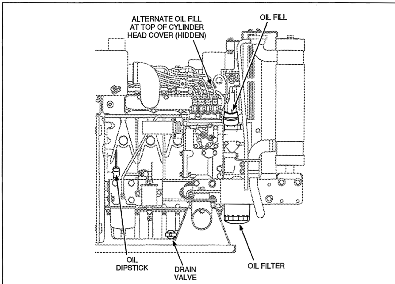
FIGURE 4. ENGINE OIL
