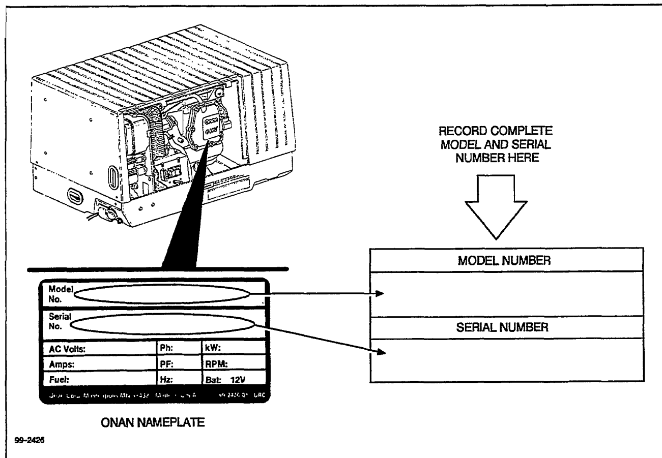
FIGURE 1. MODEL IDENTIFICATION
