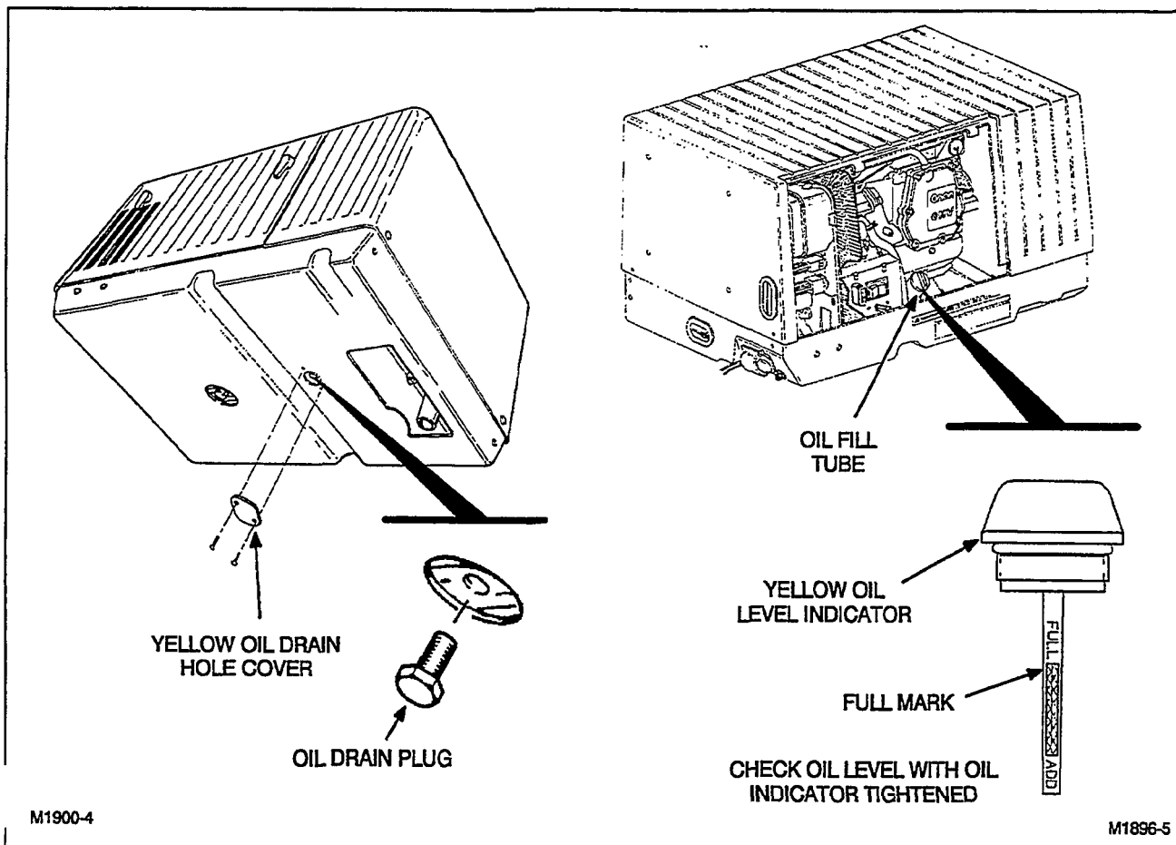
FIGURE 9. OIL CHANGE
