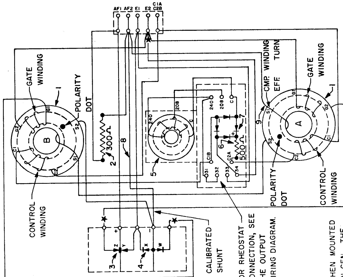
PICTORIAL
