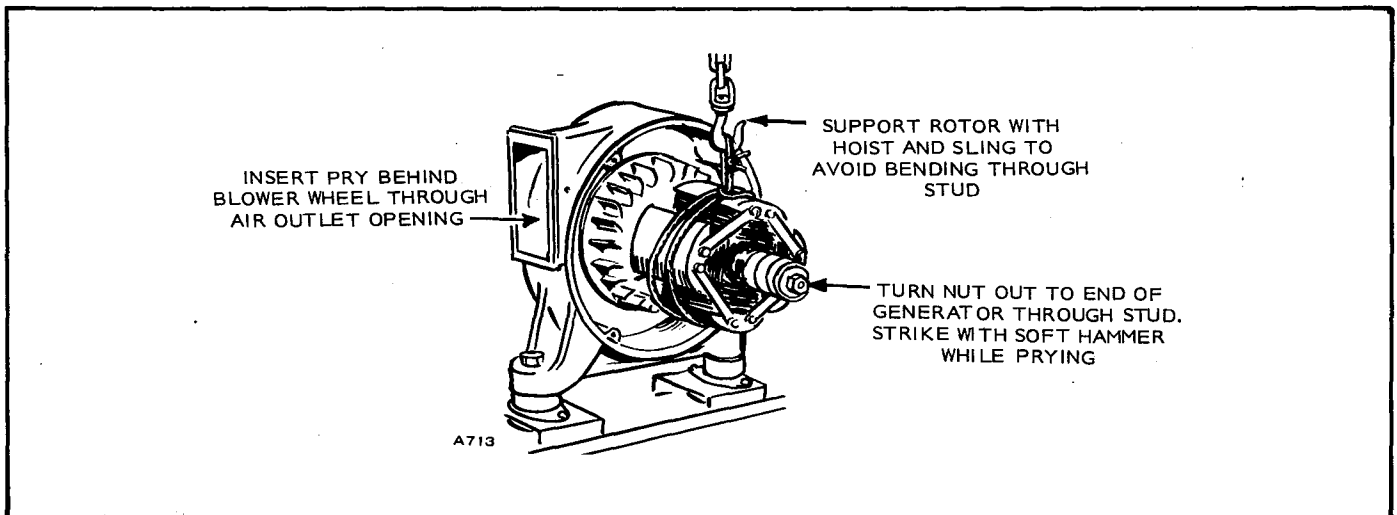
FIGURE 4-13. SUPPORTING THE ROTOR
