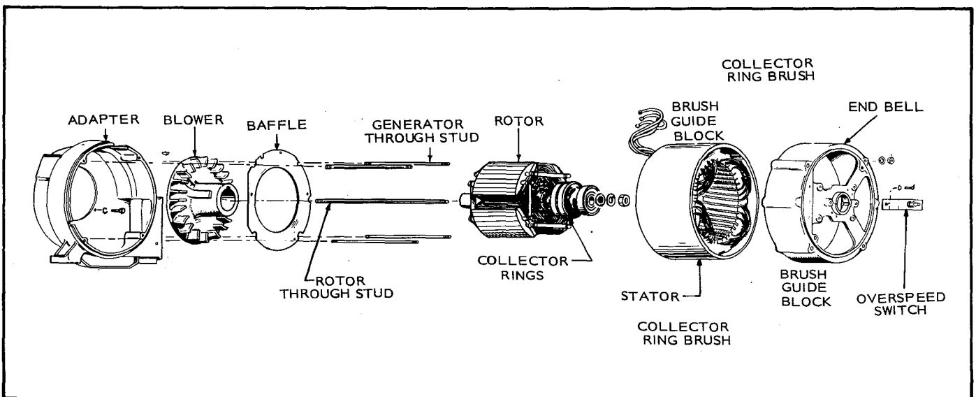
FIGURE 4-14. REVOLVING FIELD GENERATOR ASSEMBLY.
