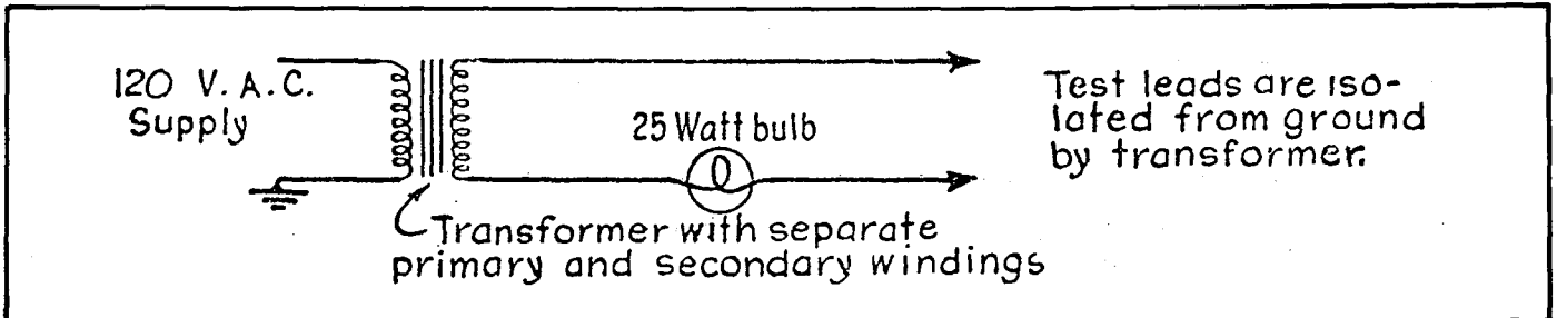
FIGURE 4-4. RECOMMENDED TEST LAMP SET
