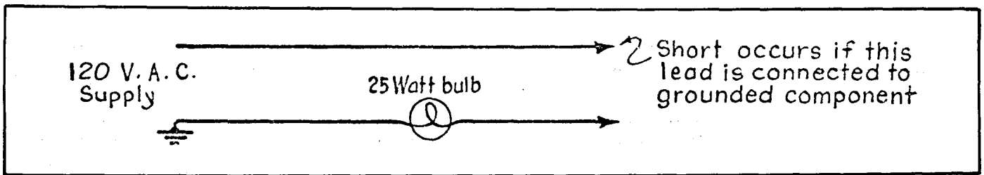
FIGURE 4-3. TEST LAMP SET
